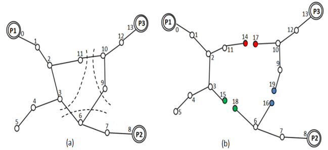
Figure 1: Multi-region decomposition of a power network using colored relay nodes on the right
