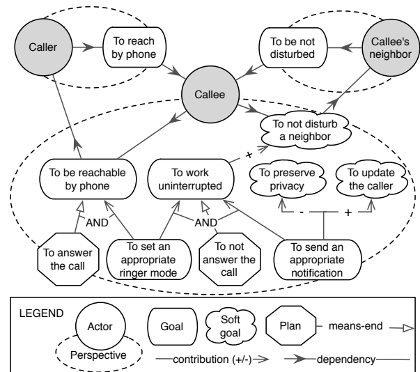
Figure 1: A Tropos system-as-is model of the ringer manager, expanding the callee’s perspective [17].
