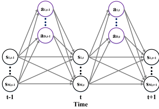
Figure 1: Graph representation of an MDP
