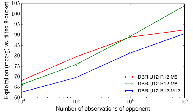
Figure 2: Impact of quantity of observations and model abstraction on exploitation of tilted 8-bucket equilibria. Exploitation values are in milli-big-blinds per game (mbb/g). Strategies for each data point are exploitable for 100 mbb/g in the 12-bucket abstract game.
