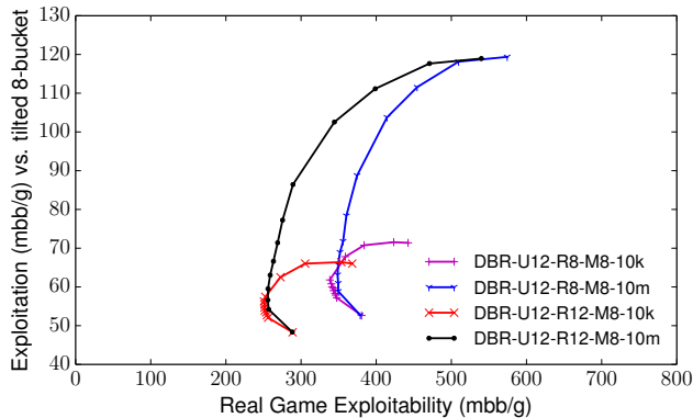
Figure 4: Impact of opponent response abstraction size and quantity of observations on DBR one-on-one and worst-case performance in the unabstracted game. Values are in milli-big-blinds per game (mbb/g).
