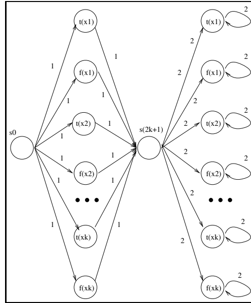
Figure 4: Reduction for Theorem 4.
