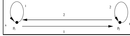
Figure 1: The resource control running example.
