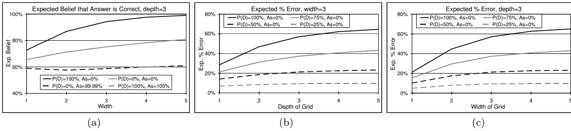
Figure 6: Expected belief and percent error for grid models of different width and depth. P(D) is the actual dependence between the nodes, while As is the assumption made about the level of independence. P(D) = 100\% means that the nodes are completely dependent, and an As = 0\% means that agents are assuming that P(D) = 0\% . (a) The expected belief that the system gives is correct, which is also the expected confidence. (b) The expected percent error as depth increases. (c) The expected percent error as width increases. The parameters used for these charts are W = 0.5 , D^p = 0.5 , B = 0.6 , I^1 = 0.2 , I^2 = 0.1 , C^1 = 0.4 , C^2 = 0.3 .
