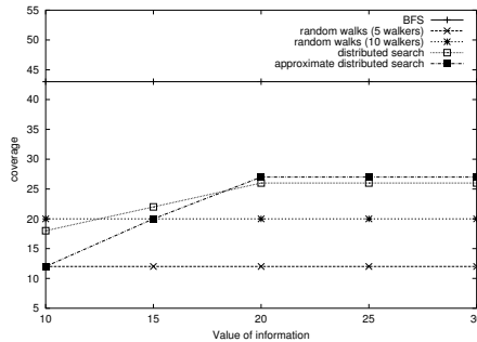
Figure 3: Comparing the coverage in experiments for a single provider ( M = 1, N = 50, c = 0.15 )
