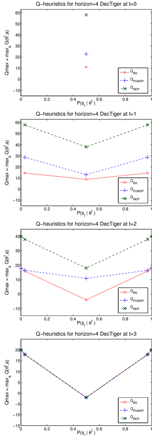
Figure 2: Q-values for horizon 4 Dec-Tiger. For each \bar{\theta}^t , corresponding to some P(s_l|\bar{\theta}^t) , the maximal Q(\bar{\theta}^t, \mathbf{a}) -value is plotted.
