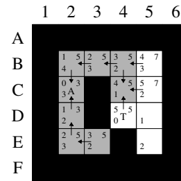
Figure 7: A*
