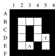
Figure 1: Gridworld
