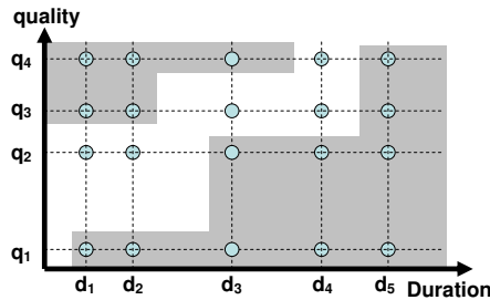
Figure 2: A method's outcome space
