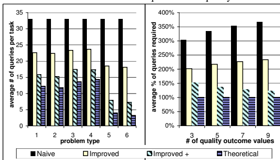
Figure 3: # of interactions initiated
