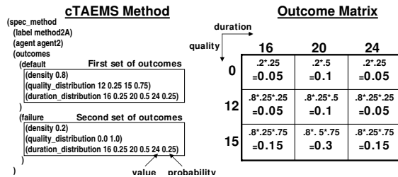
Figure 1: A typical method in cTAEMS
