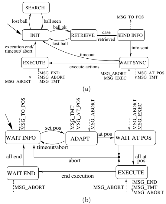
Figure 2: (a) Retriever/coordinator behavior. (b) Default behavior.
