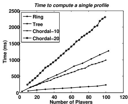
Figure 3: Repeated prisoner’s dilemma results. This graph shows the time taken by PureProp-R to find a single feasible and \epsilon -enforceable profile. In the repeated setting too, the complexity is roughly linear in the number of players and is more strongly affected by graph density.
