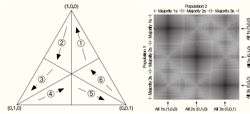
Figure 1: The projection of \Delta^3 \times \Delta^3 to [0, 1]^2 . (left): The projection divides the simplex \Delta^3 into six equal-area triangles; arrows shows the direction for sorting points in each area. (right): Visualization of the cartesian product of two simplices.
