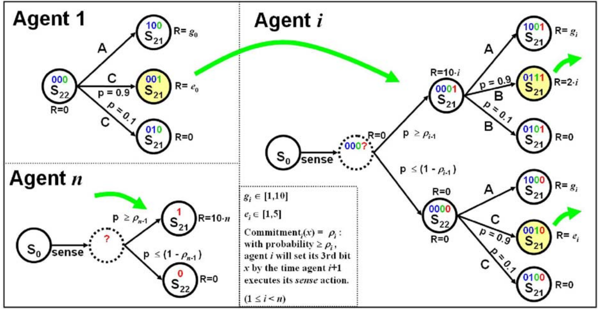
Figure 2: n -agent Commitment Chain problem.
