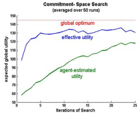
Figure 3: 5-agent Commitment Chain Results
