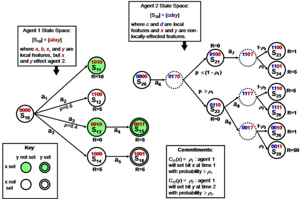
Figure 1: Simple local MDP models with non-local effects and commitments between 2 agents.
