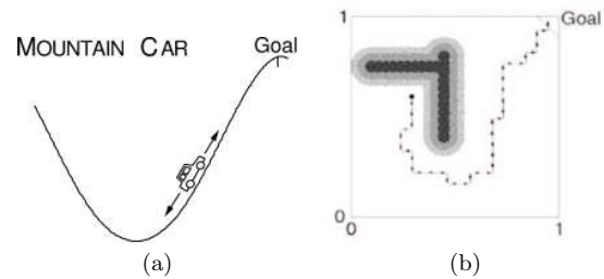
Figure 3: Two of the domains from the NIPS benchmarking workshop: (a) Mountain Car and (b) Puddle World.
