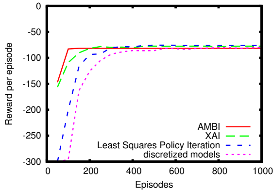
Figure 4: Learning curves for Mountain Car
