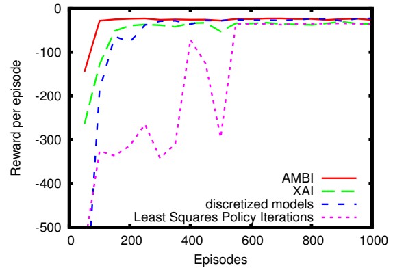
Figure 5: Learning curves for Puddle World
