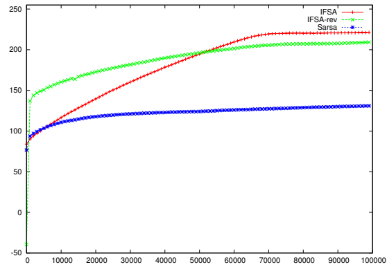
Figure 3: IFSA outperforms the base learning algorithm in Gridworld significantly, regardless of the ordering of the state features in \Phi .
