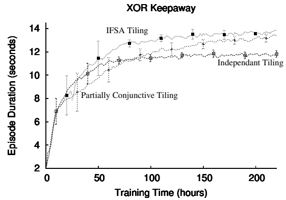
Figure 8: IFSA outperforms learning with just \phi_0 (independent tiling) and learning with \phi_0 and \phi_1 (partially conjunctive tiling) from the start. 10 independent learning curves for each of the three setups are averaged and error bars show the standard deviation.
