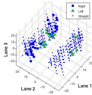
Figure 7: Driving training data demonstrating the agent's driving policy in the middle lane. Graph axes represent distance to the nearest car in each of the three driving lanes.
