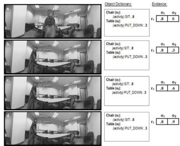
Figure 8: The correction of a false positive caused by a misleading cue.
