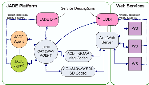
Figure 1: WSIG Architecture
