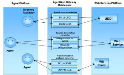
Figure 2: AgentWeb Gateway Architecture
