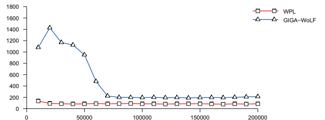
Figure 3: Comparing the average total service time for 200,000 time steps of the DTAP problem for WPL and GIGA-WoLF.
