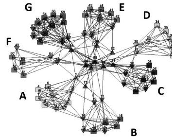
Figure 1: Example Afghani leadership network
