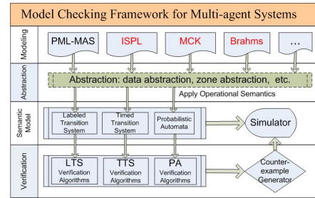
Figure 3: Architecture of the Model Checker Framework
