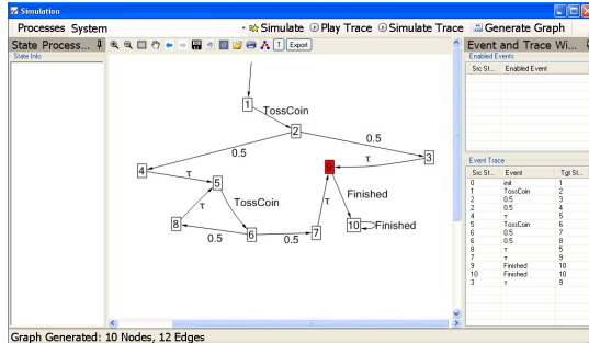
Figure 2: Simulator of the Model Checker Framework
