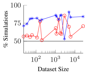
Figure 2: Accuracy
